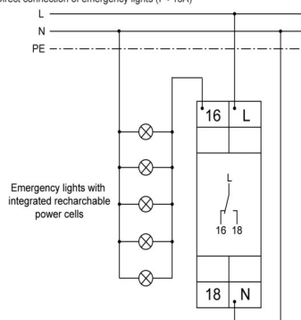
Direct connection of emergency lights (I < 16A)
