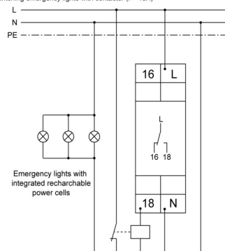
Switching emergency lights with contactor (I > 16A)
